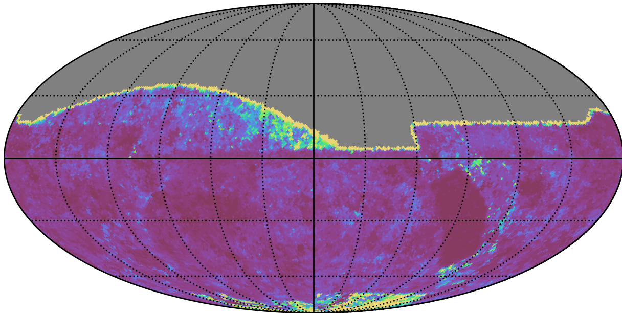
baseline_v2.1_10yrs All sky g band: 20thPercentile Inter-Night Gap
