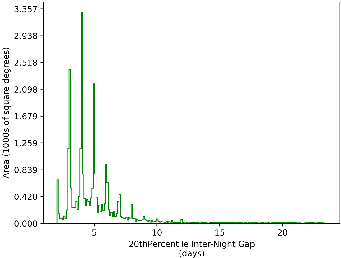
baseline_v2.1_10yrs All sky g band: 20thPercentile Inter-Night Gap
