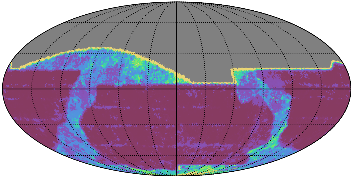
baseline_v2.1_10yrs All sky all bands: 20thPercentile Inter-Night Gap
