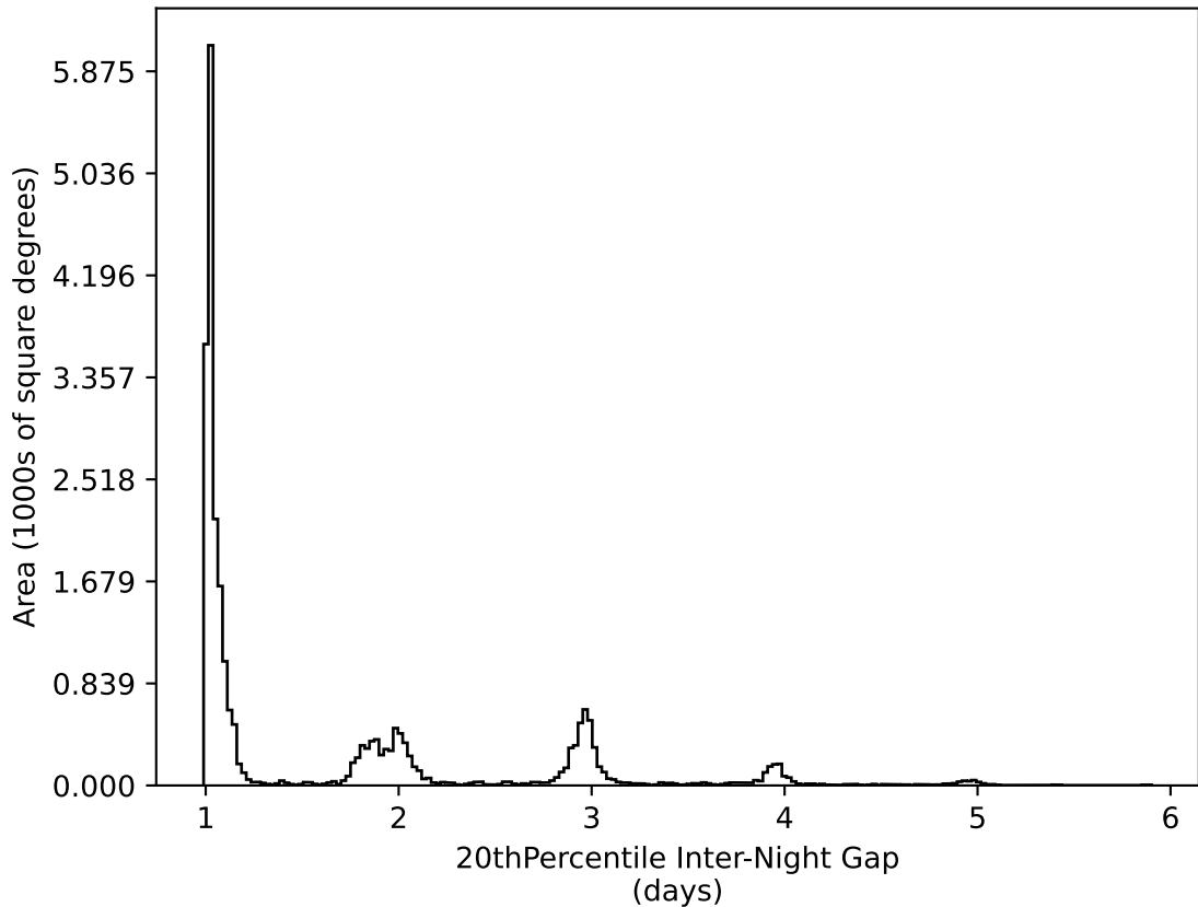
baseline_v2.1_10yrs All sky all bands: 20thPercentile Inter-Night Gap
