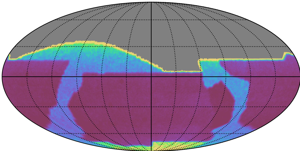
baseline_v2.1_10yrs : properMotion
