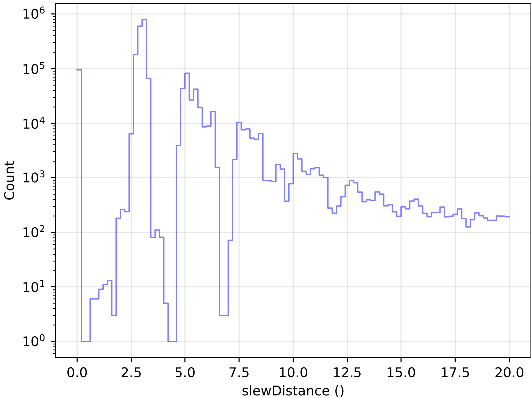
baseline_v2.1_10yrs All visits: Zoom Slew Distance Histogram
