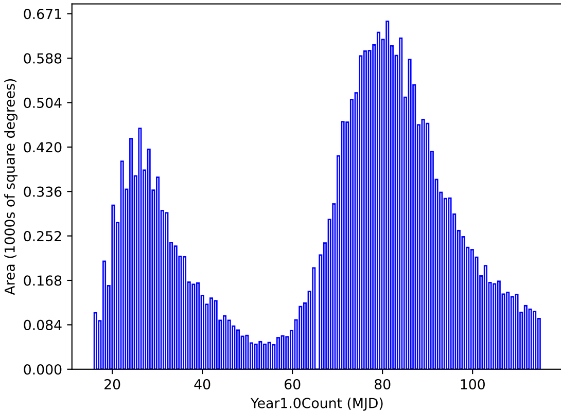
baseline_v2.1_10yrs night < 365.25: Year1.0Count
