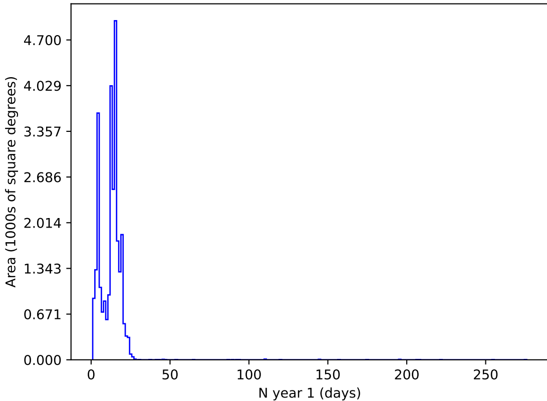
baseline_v2.1_10yrs z and night < 365: N year 1
