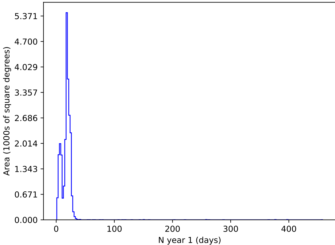
baseline_v2.1_10yrs y and night < 365: N year 1
