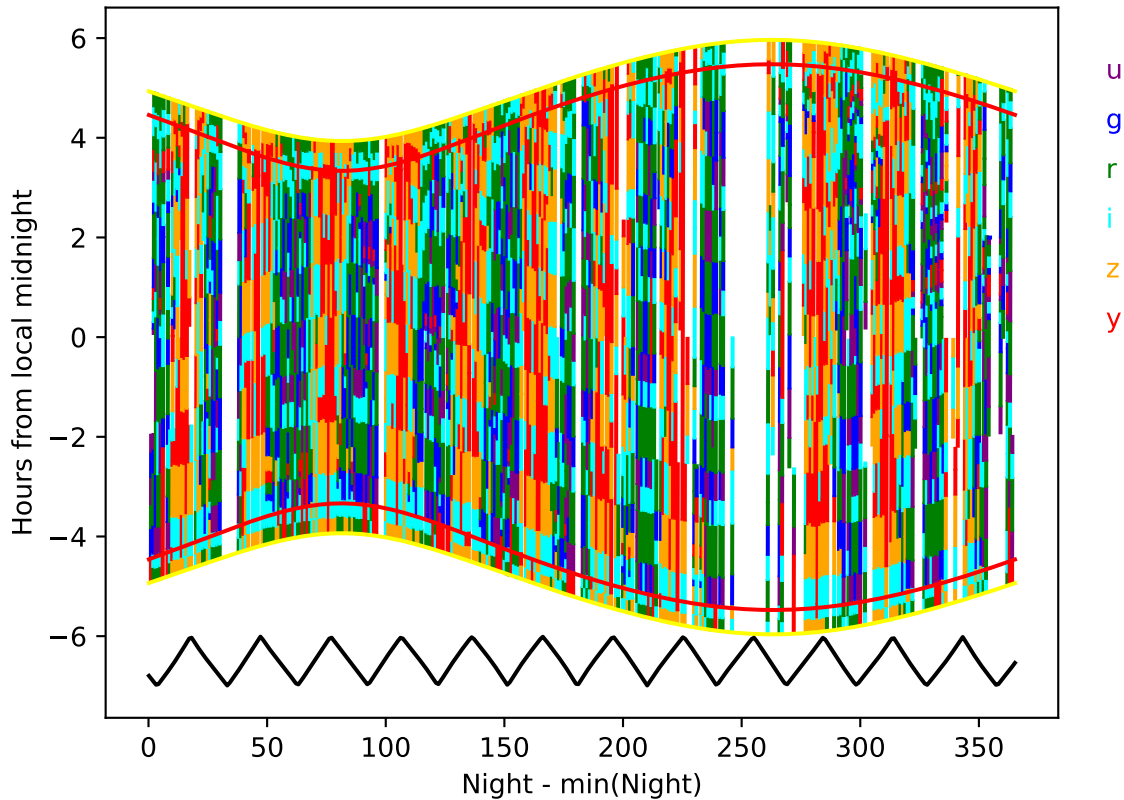
baseline_v2.1_10yrs year 9-10: Hourglass
