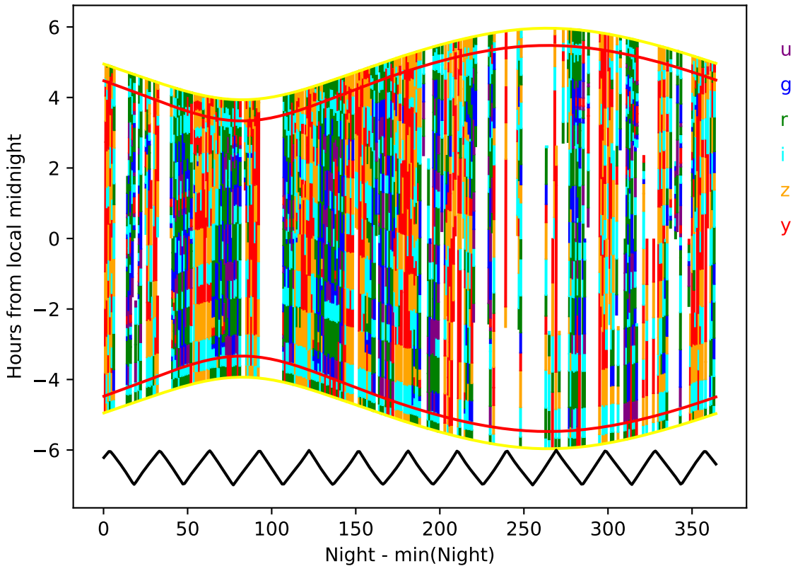
baseline_v2.1_10yrs year 5-6: Hourglass
