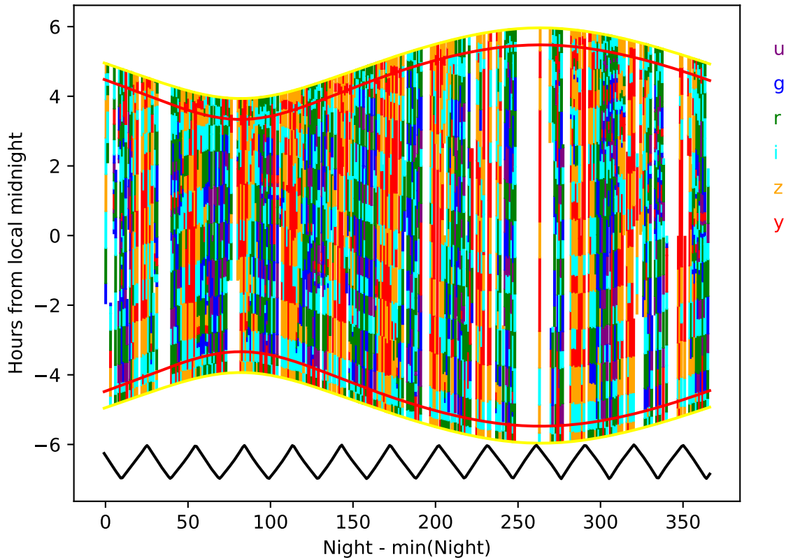
baseline_v2.1_10yrs year 3-4: Hourglass
