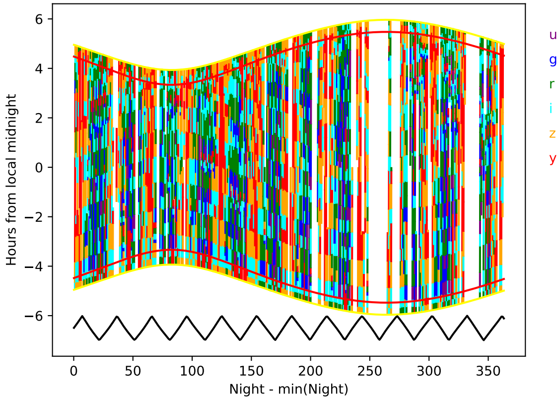
baseline_v2.1_10yrs year 2-3: Hourglass
