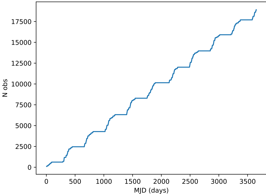
baseline_v2.1_10yrs note like DD:XMM_LSS%: Cumulative
