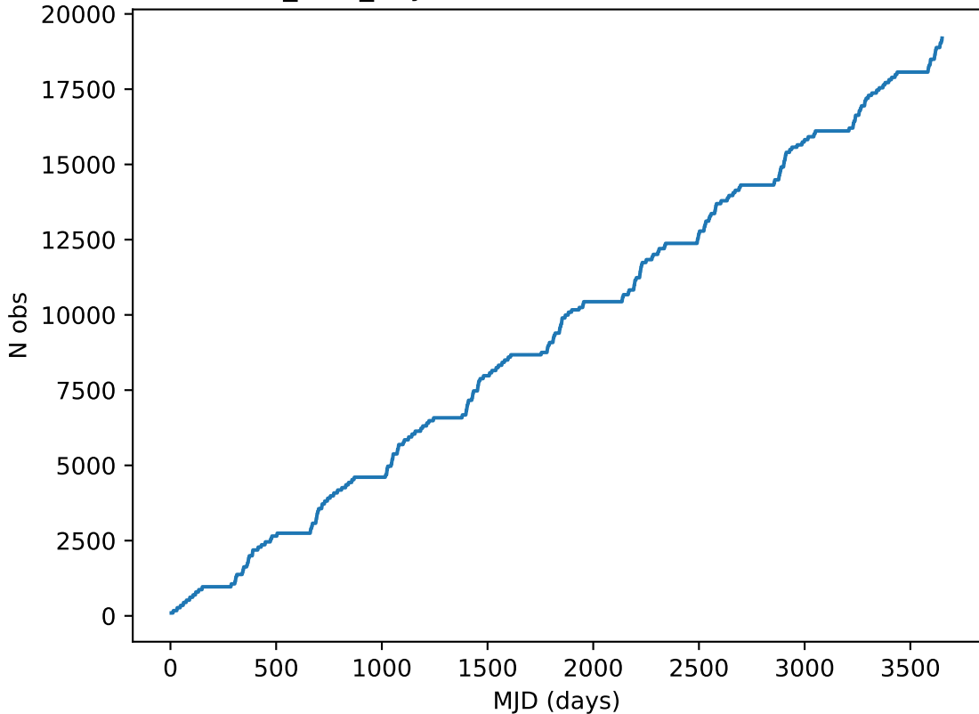
baseline_v2.1_10yrs note like DD:ECDFS%: Cumulative
