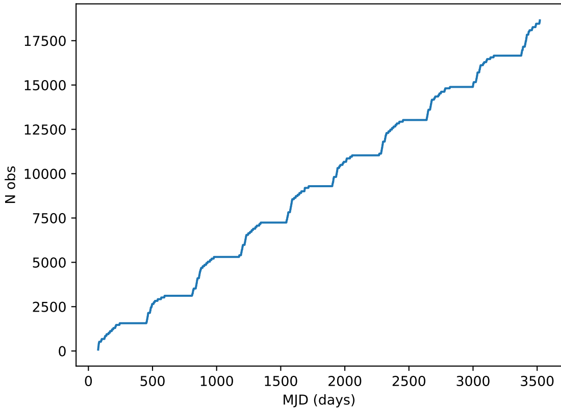
baseline_v2.1_10yrs note like DD:COSMOS%: Cumulative
