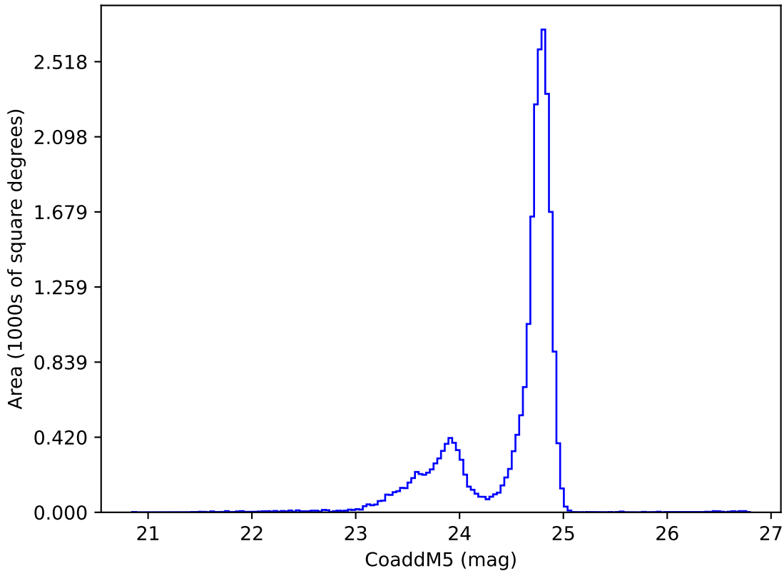
baseline_v2.1_10yrs y: CoaddM5
