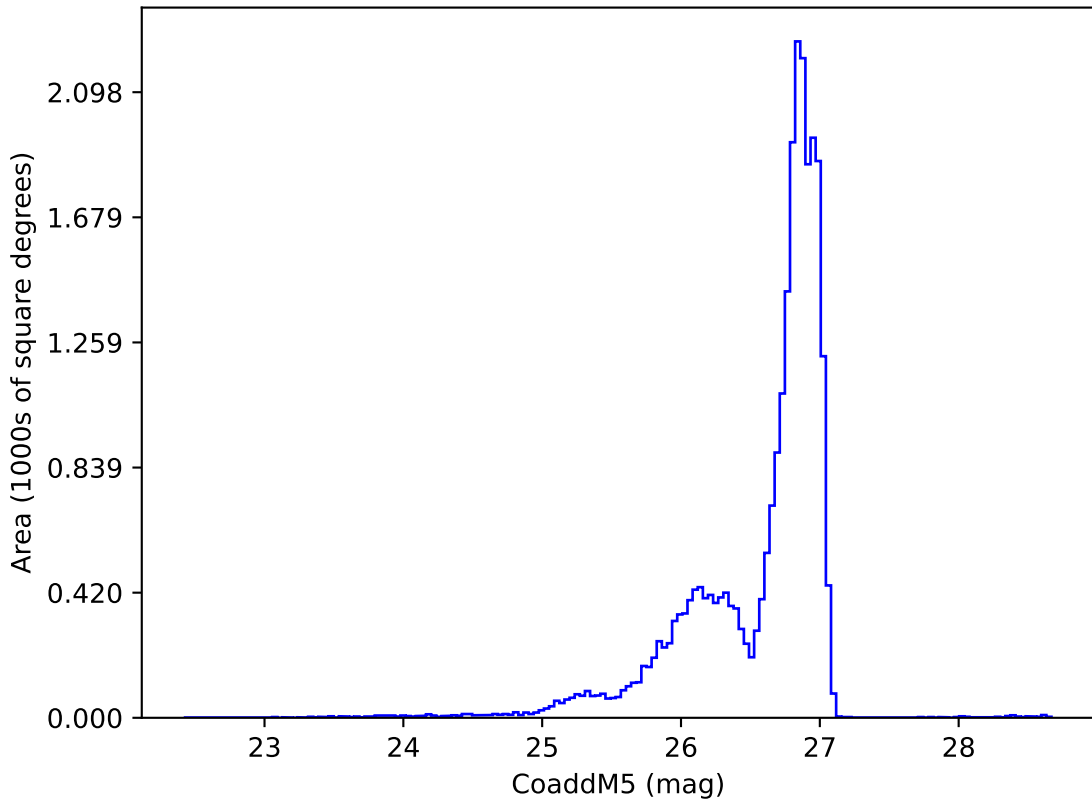
baseline_v2.1_10yrs r: CoaddM5
