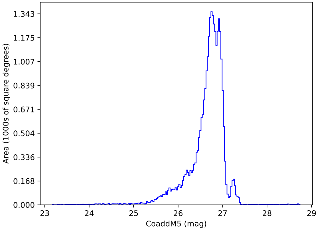
baseline_v2.1_10yrs g: CoaddM5
