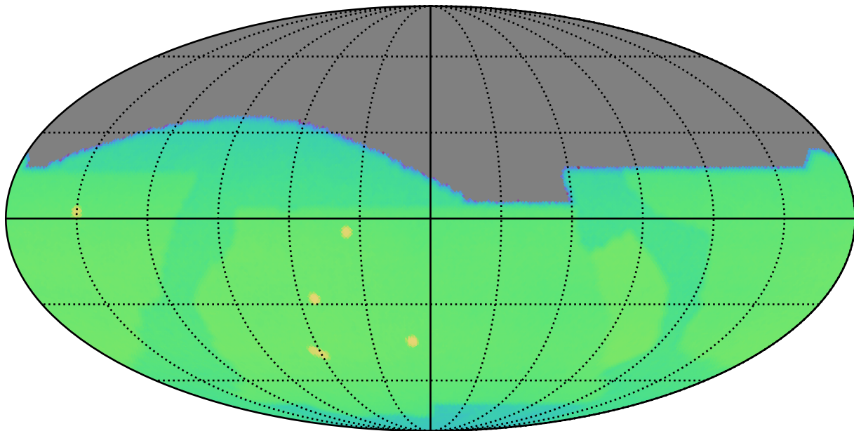
baseline_v2.1_10yrs : CoaddM5
