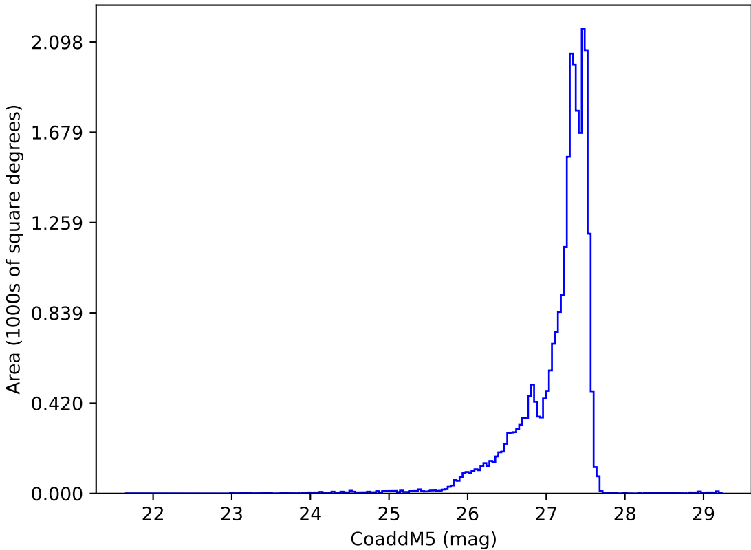
baseline_v2.1_10yrs : CoaddM5
