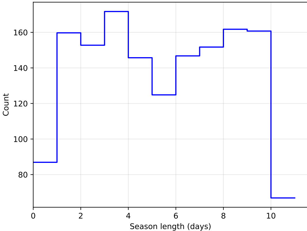
baseline_v2.1_10yrs DD:XMM_LSS all bands: SeasonLength
