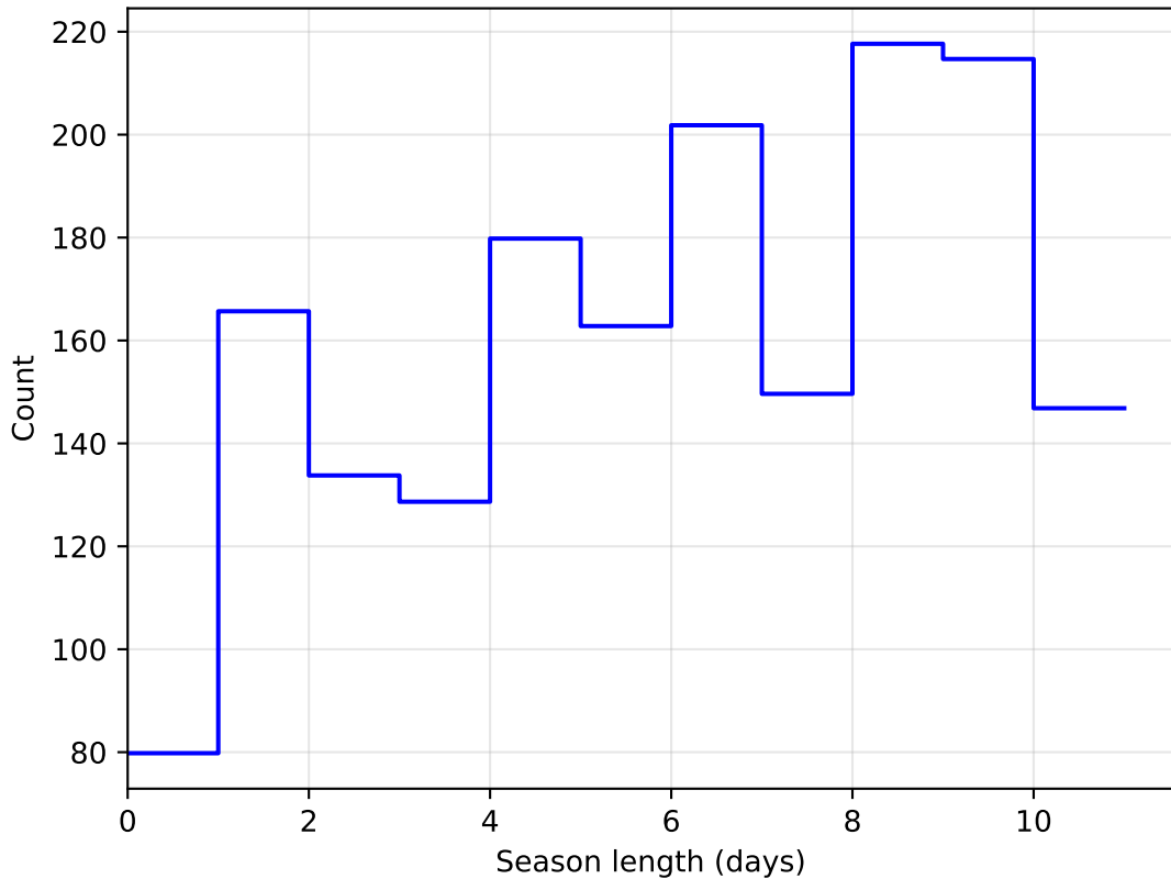
baseline_v2.1_10yrs DD:WFD all bands: SeasonLength
