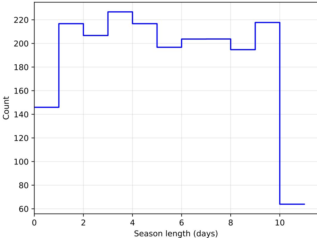
baseline_v2.1_10yrs DD:ECDFS all bands: SeasonLength
