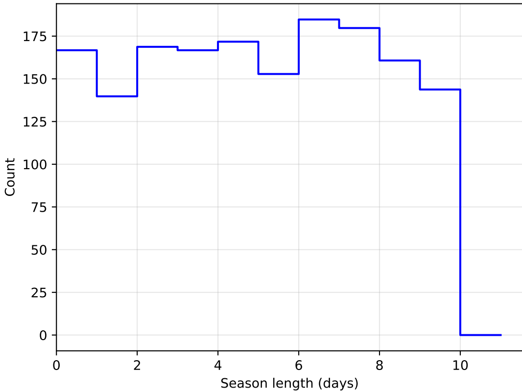
baseline_v2.1_10yrs DD: COSMOS all bands: SeasonLength
