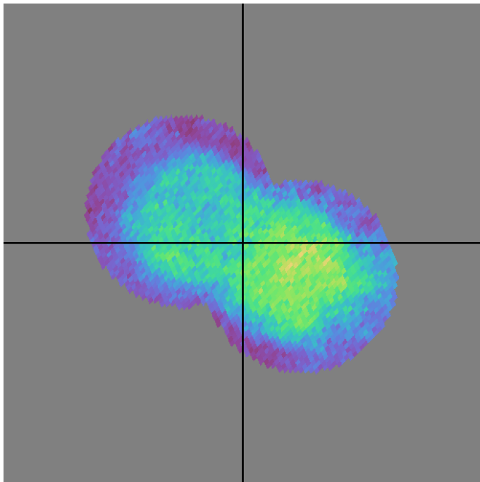
baseline_v2.1_10yrs DD:EDFS all bands: SNSLMetric
