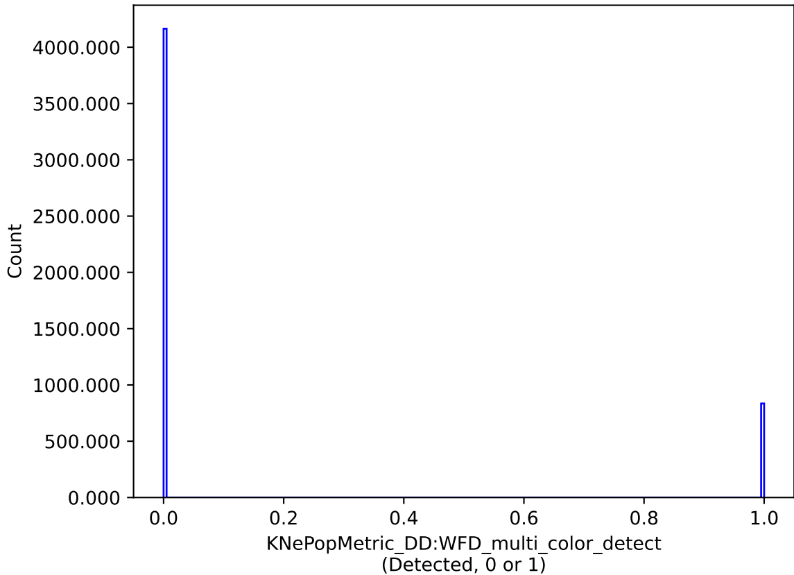
baseline_v2.1_10yrs DD:WFD: KNePopMetric_DD:WFD_multi_color_detect
