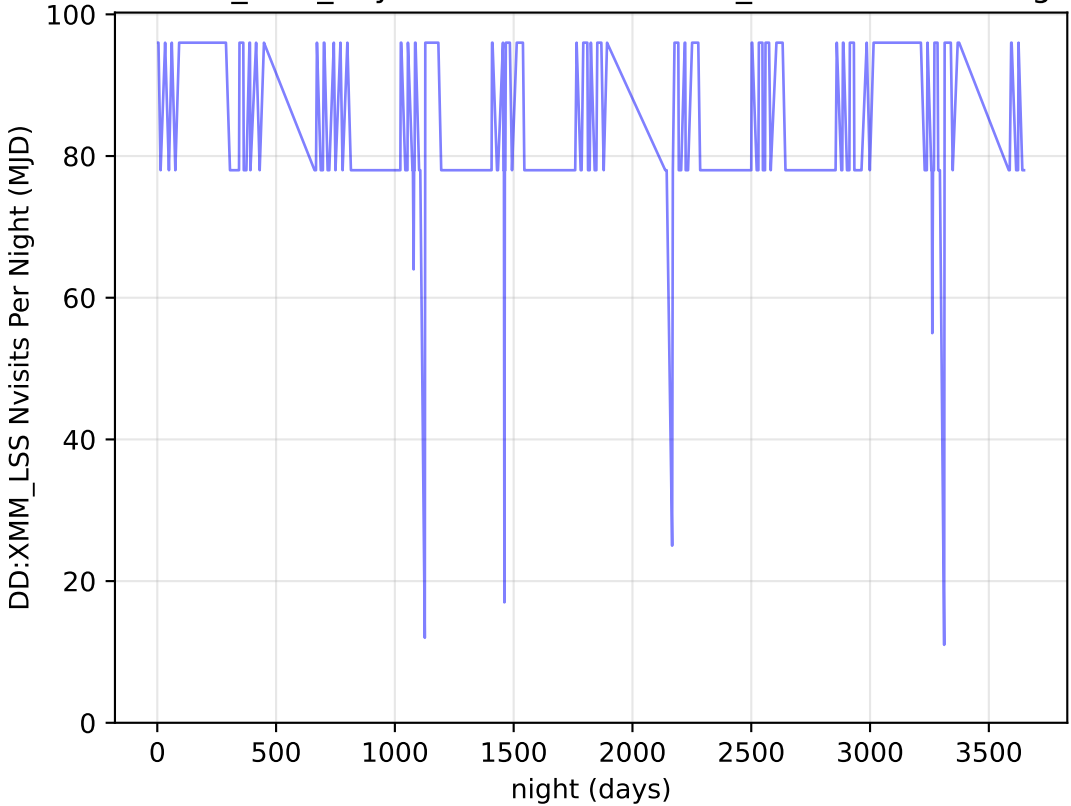
baseline_v2.1_10yrs all bands: DD:XMM_LSS Nvisits Per Night
