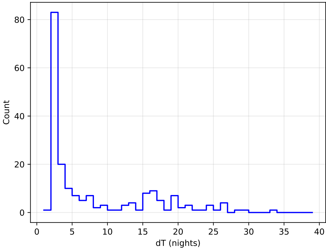
baseline_v2.1_10yrs all bands: DD:XMM_LSS Delta Nights Histogram
