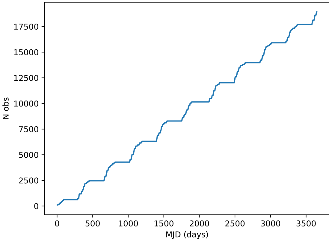
baseline_v2.1_10yrs all bands: DD:XMM_LSS Cumulative NVisits
