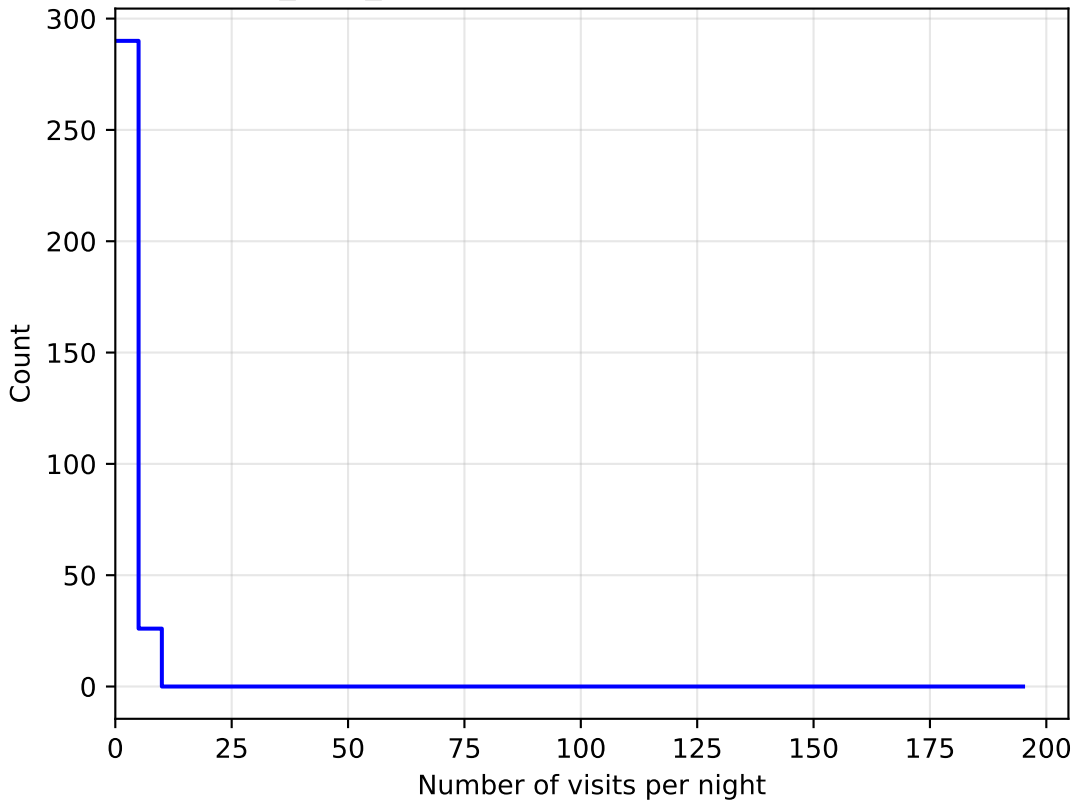
baseline_v2.1_10yrs all bands: DD:WFD NVisitsPerNight
