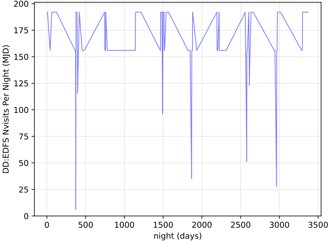
baseline_v2.1_10yrs all bands: DD:EDFS Nvisits Per Night
