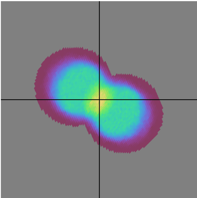
baseline_v2.1_10yrs all bands: DD:EDFS NVisits
