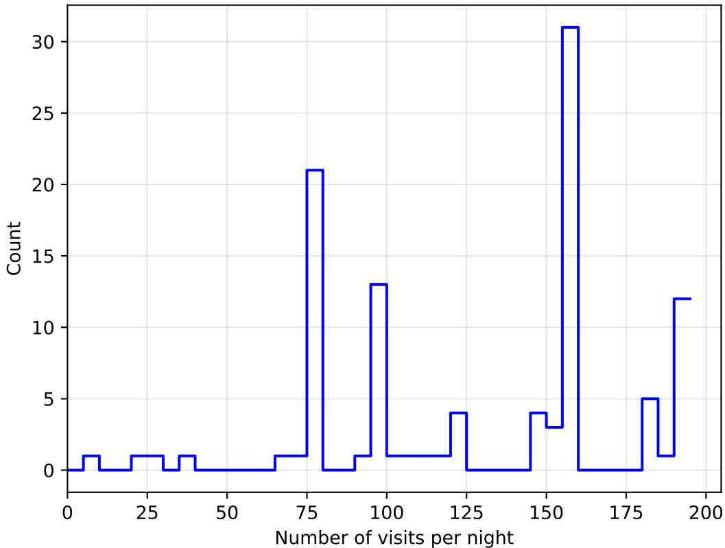
baseline_v2.1_10yrs all bands: DD:EDFS NVisitsPerNight
