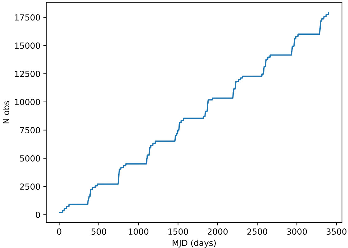
baseline_v2.1_10yrs all bands: DD:EDFS Cumulative NVisits
