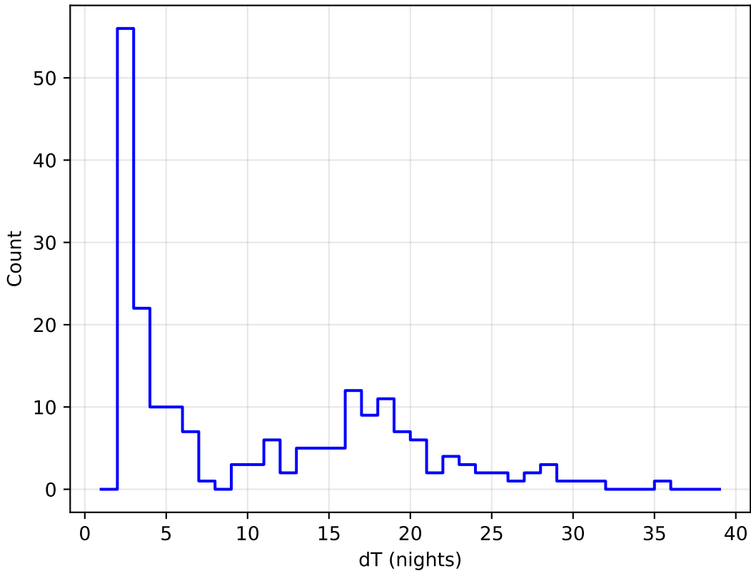
baseline_v2.1_10yrs all bands: DD:ECDFS Delta Nights Histogram
