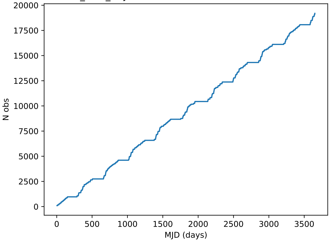
baseline_v2.1_10yrs all bands: DD:ECDFS Cumulative NVisits
