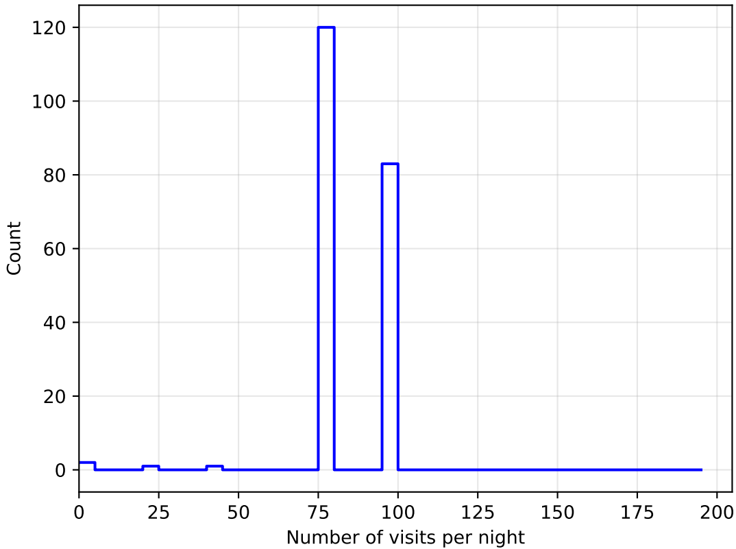
baseline_v2.1_10yrs all bands: DD: COSMOS NVisitsPerNight
