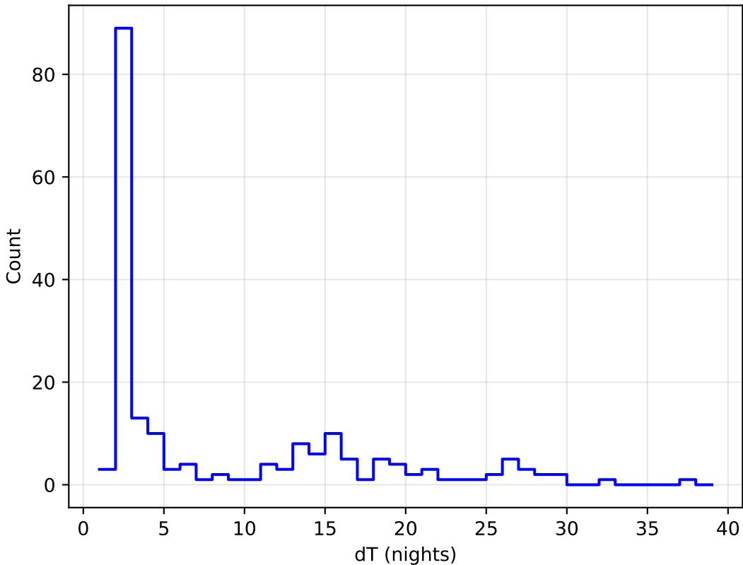
baseline_v2.1_10yrs all bands: DD: COSMOS Delta Nights Histogram
