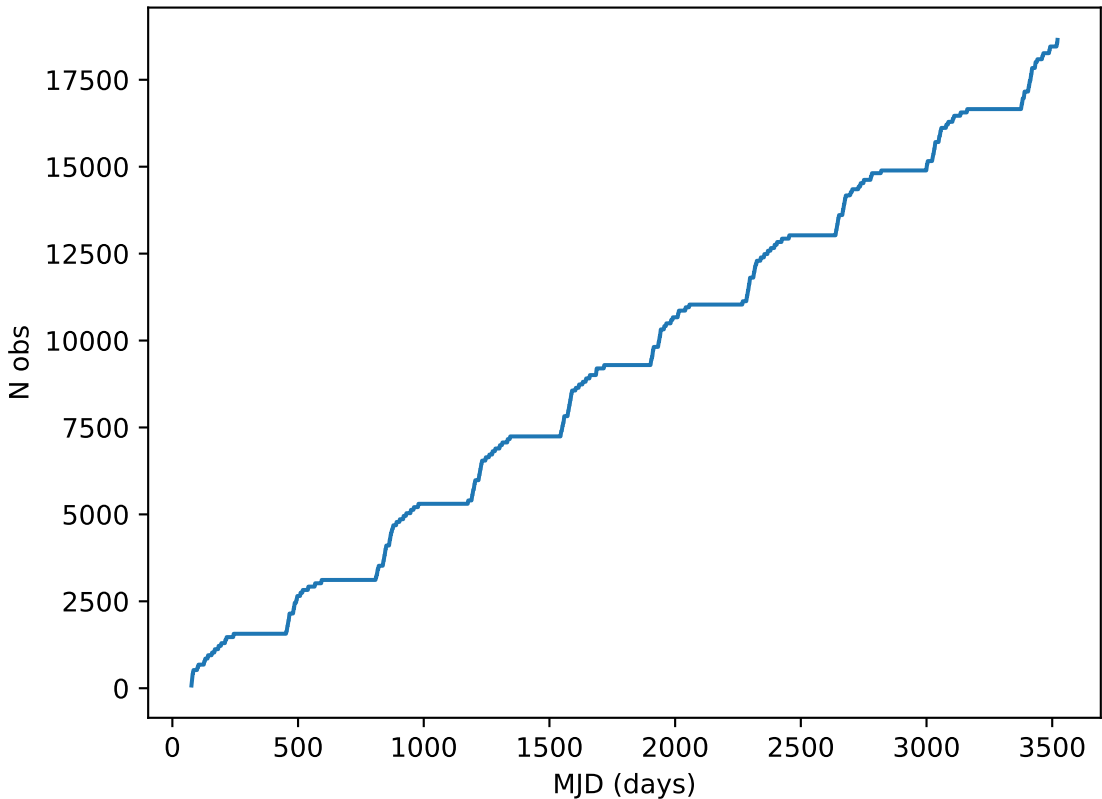
baseline_v2.1_10yrs all bands: DD: COSMOS Cumulative NVisits
