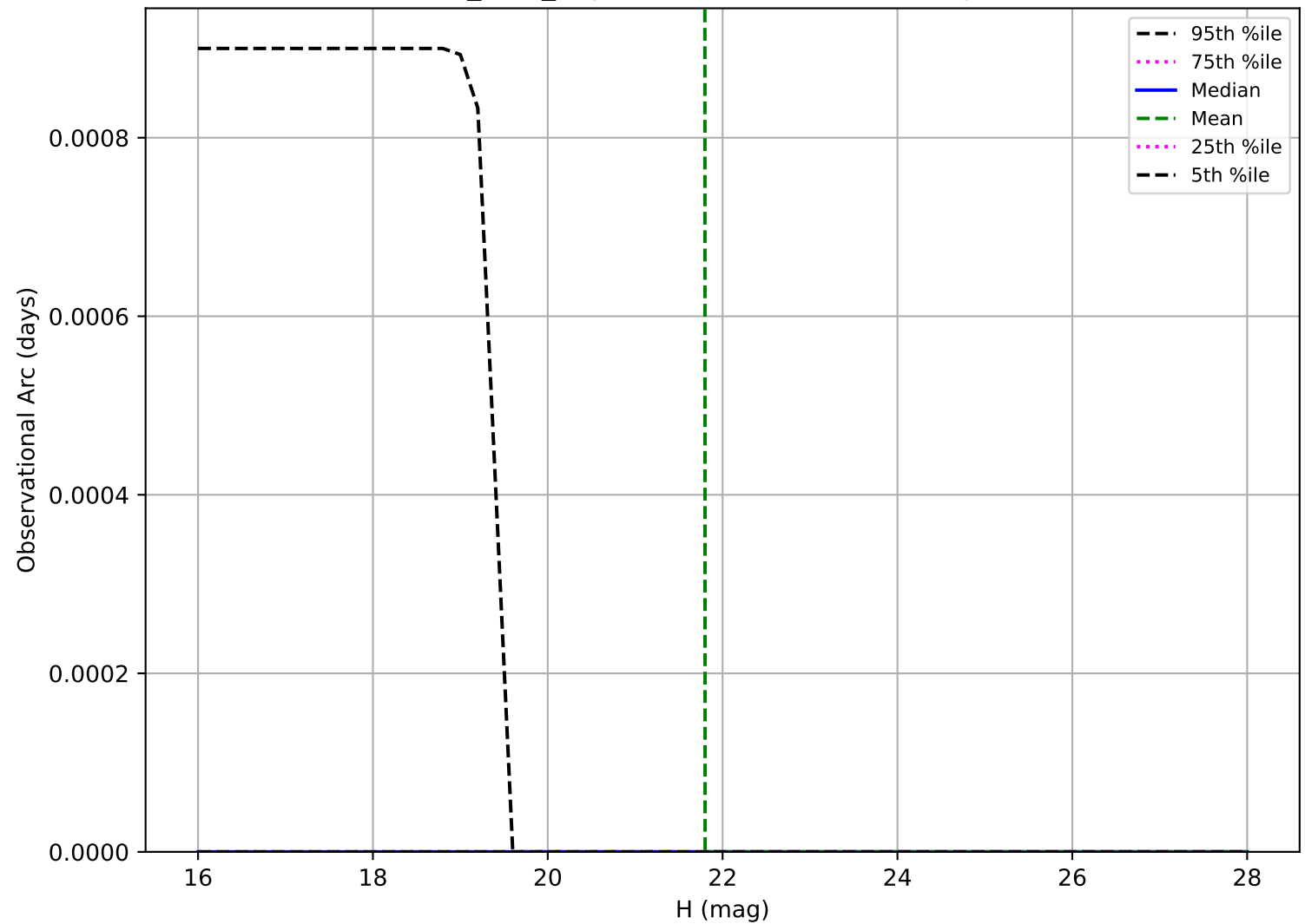
baseline_v2.0_10yrs: Observational Arc Length Vatira
