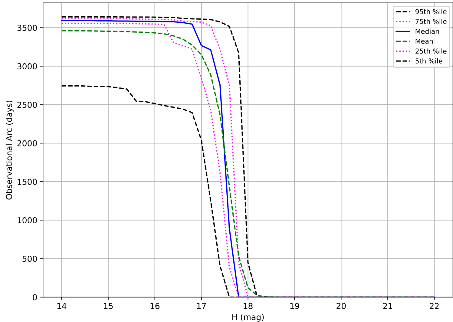
baseline_v2.0_10yrs: Observational Arc Length Trojan
