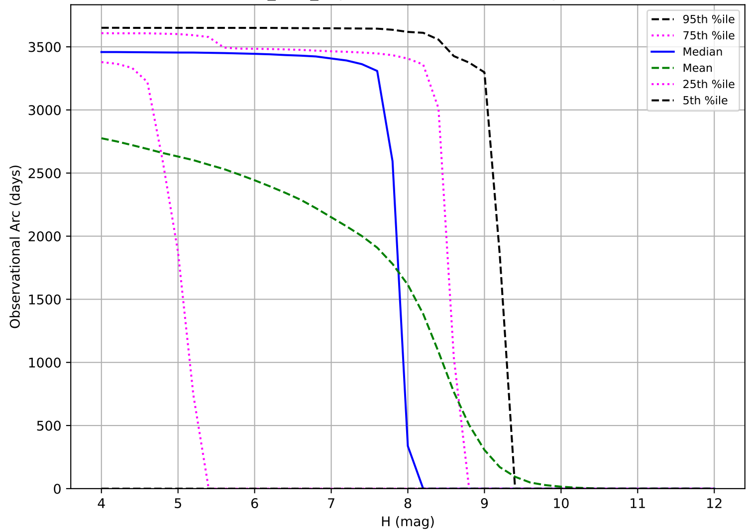
baseline_v2.0_10yrs: Observational Arc Length TNO
