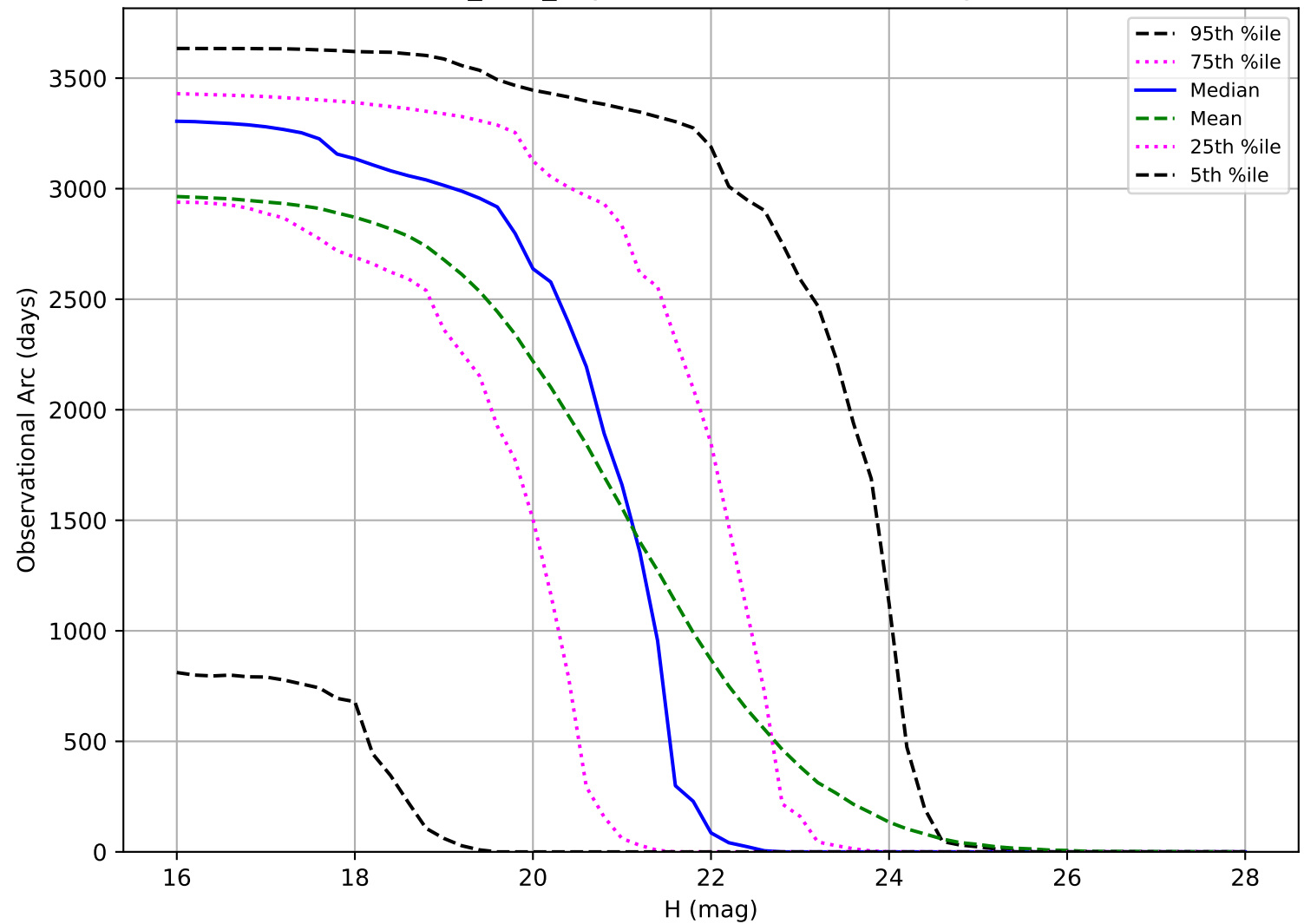
baseline_v2.0_10yrs: Observational Arc Length PHA
