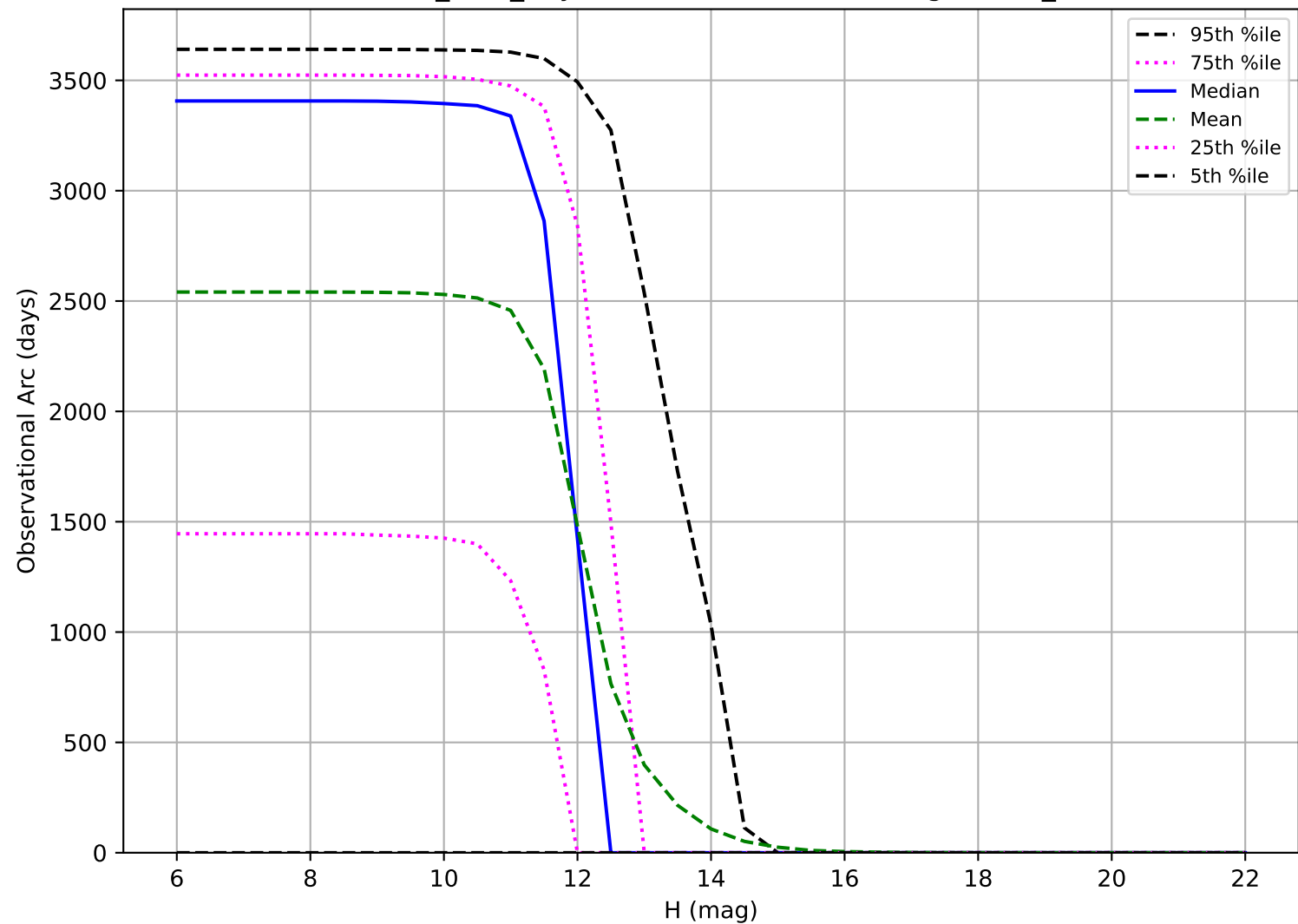
baseline_v2.0_10yrs: Observational Arc Length OCC_r20
