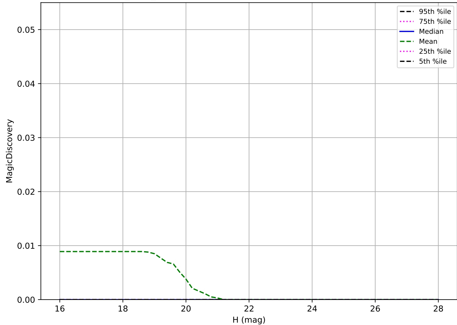
baseline_v2.0_10yrs: Vatira 6 detections in 60 nights detection loss
