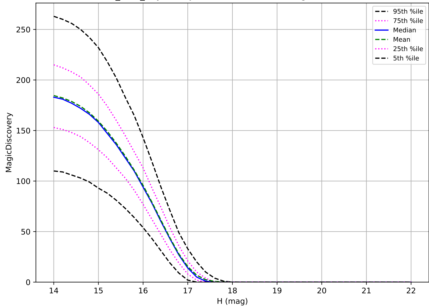
baseline_v2.0_10yrs: Trojan 6 detections in 60 nights detection loss
