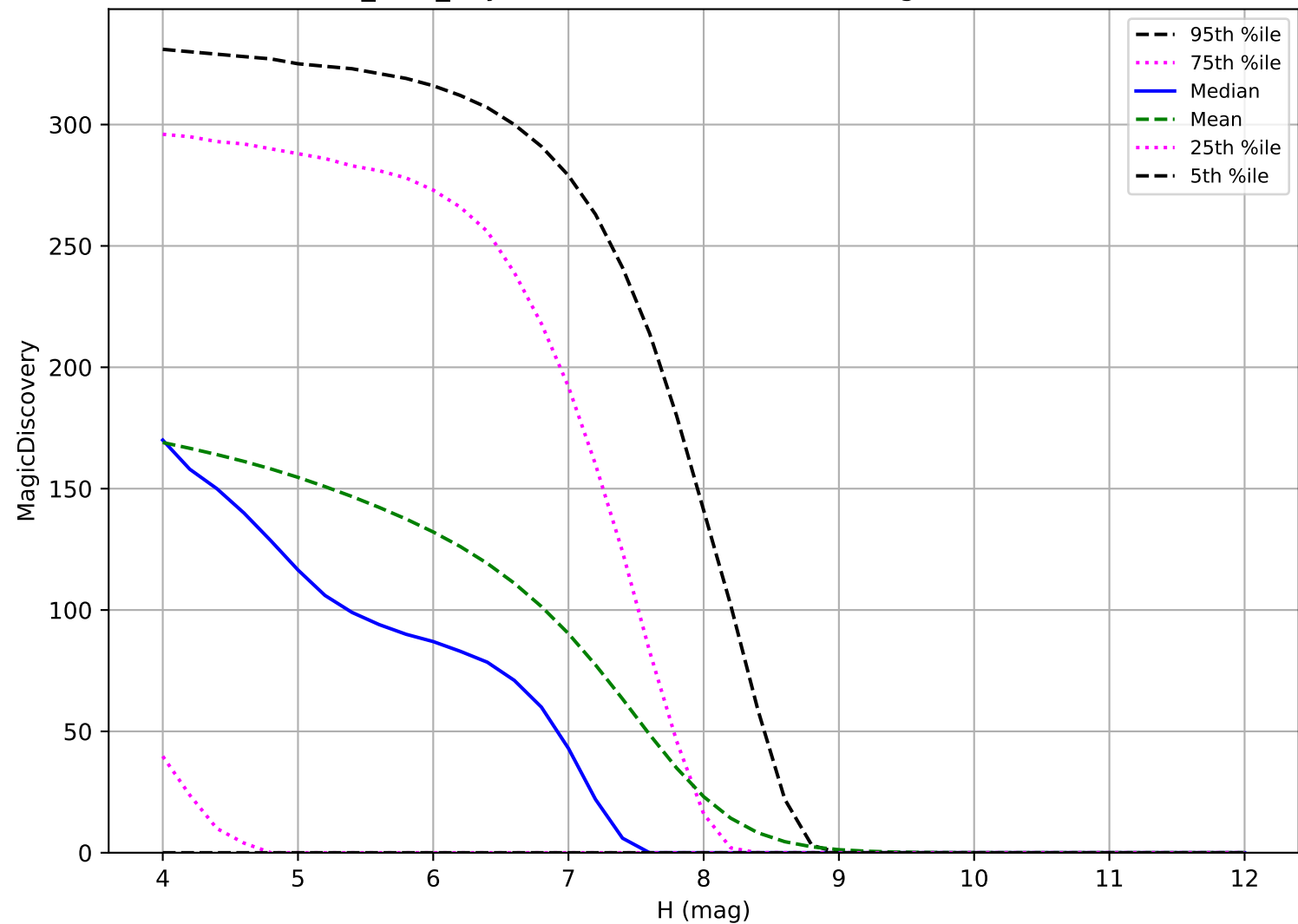
baseline_v2.0_10yrs: TNO 6 detections in 60 nights detection loss
