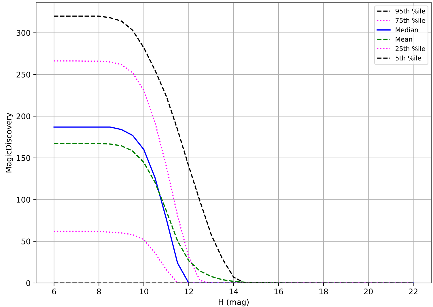
baseline_v2.0_10yrs: OCC_r20 6 detections in 60 nights detection loss
