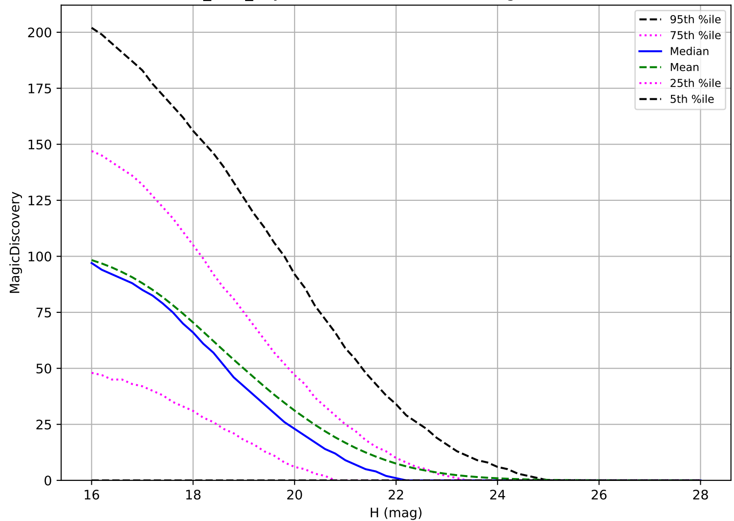
baseline_v2.0_10yrs: NEO 6 detections in 60 nights detection loss
